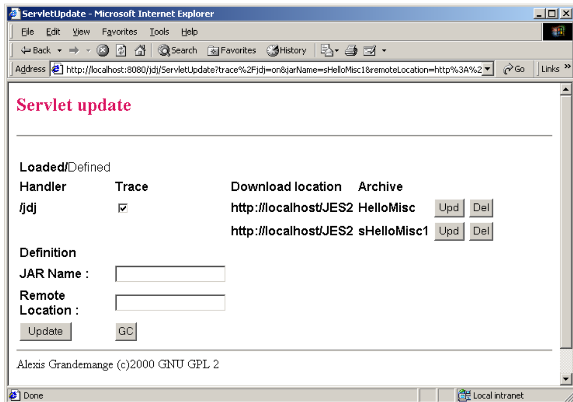
Figure 7: ServletUpdate list
