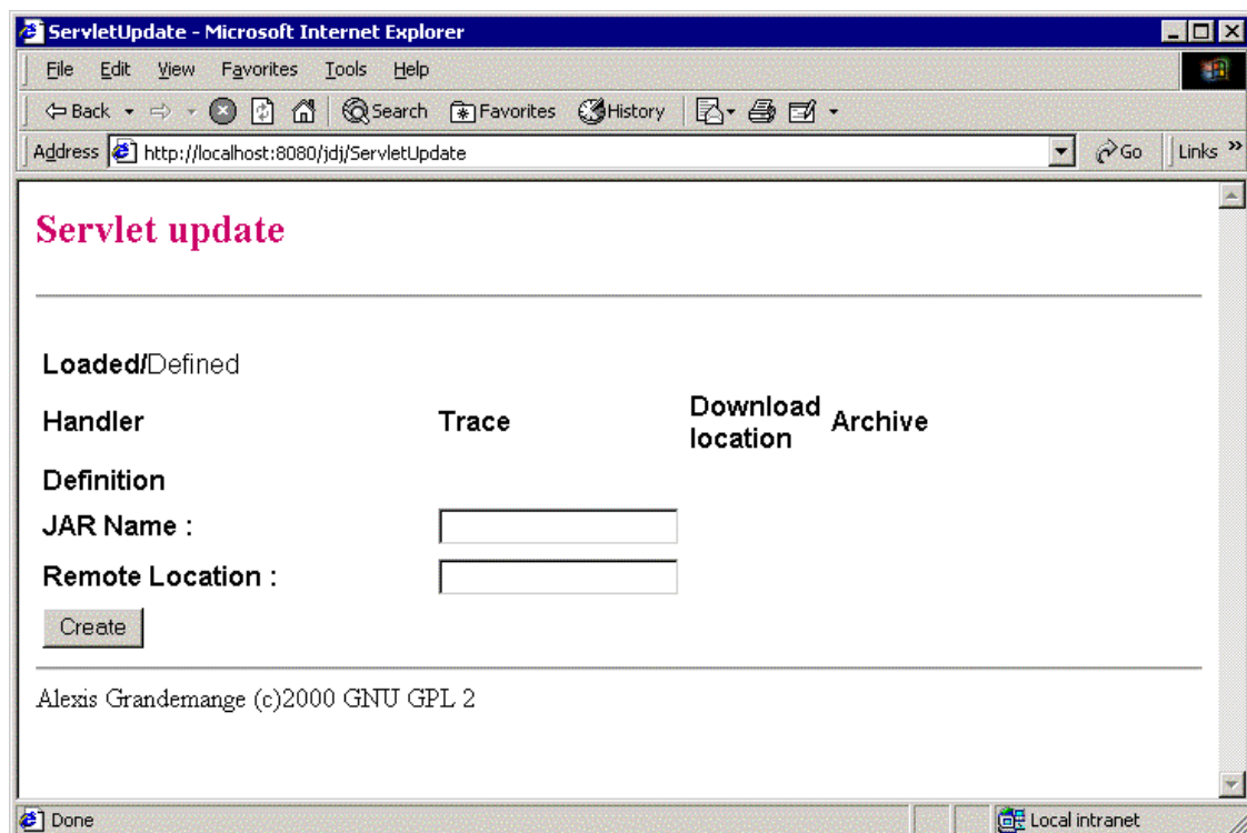
Figure 6: ServletUpdate definition
